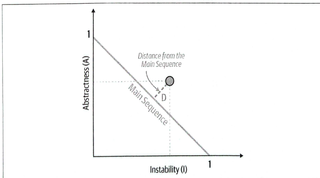
Figure 3-3. Normalized Distance from the Main Sequence for a particular class
