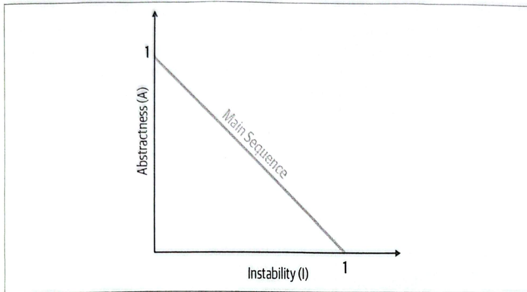
Figure 3-2. The main sequence defines the ideal relationship between Abstractness and Instability
